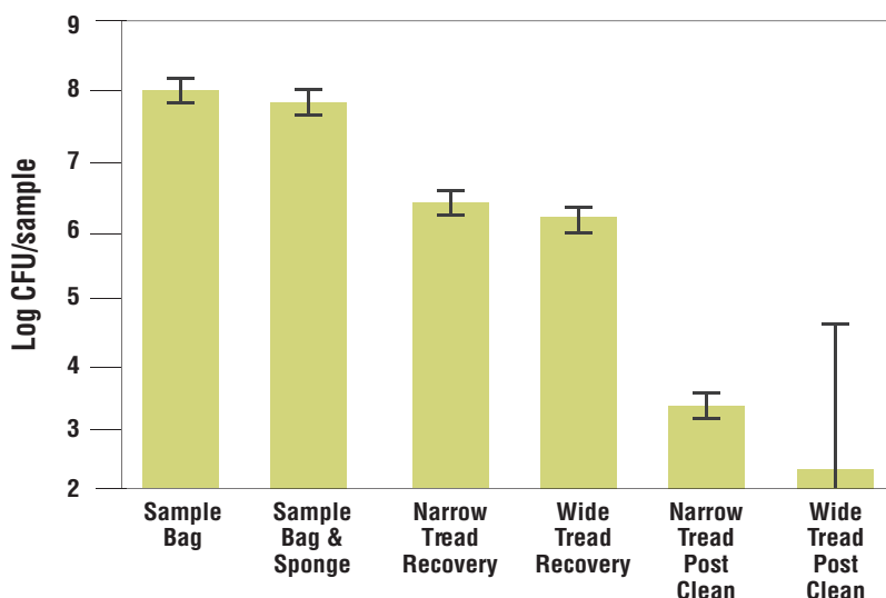
Figure 3. Populations (log CFU/sample) of a multi-species Gram-negative inoculum recovered from sample bags, sample bags including a sponge, sponges following sampling narrow-tread boots, sponges following sampling wide-tread boots, and sponges following sampling inoculated narrow- and wide-tread boots after cleaning and disinfection. Interval bars represent 95% CI for the means
